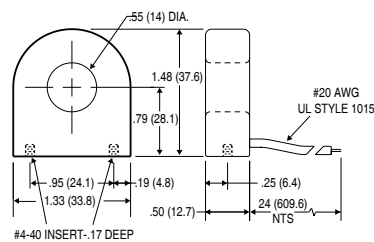
Model 18 Dimensions
